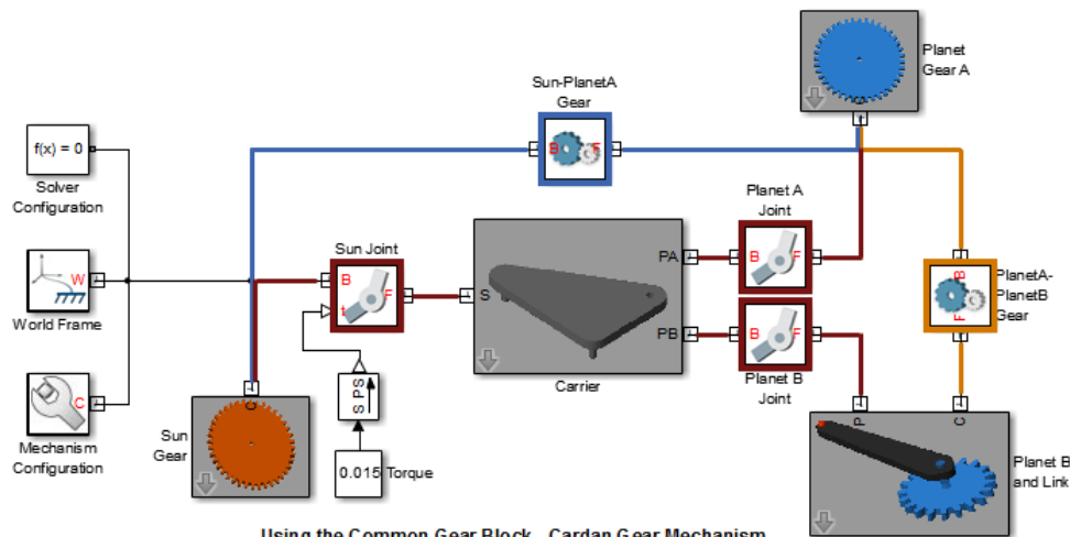
This example shows the Cardan Gear mechanism that converts rotational motion into reciprocating linear motion without using linkages or sliders. The mechanism uses three gears - one sun and two planet gears. The sun gear is twice as large as the planet gears (which are of the same size). The red pointer on the link traces a straight line as the gears rotate.
